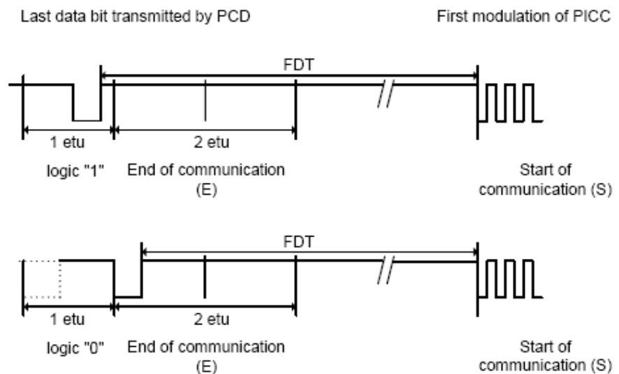
Fig. 12 Frame delay time PCD to PICC
