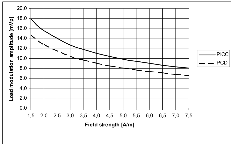
Fig. 14: Load modulation amplitude as a function of field strength
