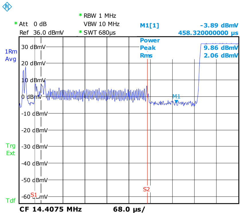
Fig.18 EMD measurement - time domain power (ISO/IEC 14443 Type B 106 kbit/)
