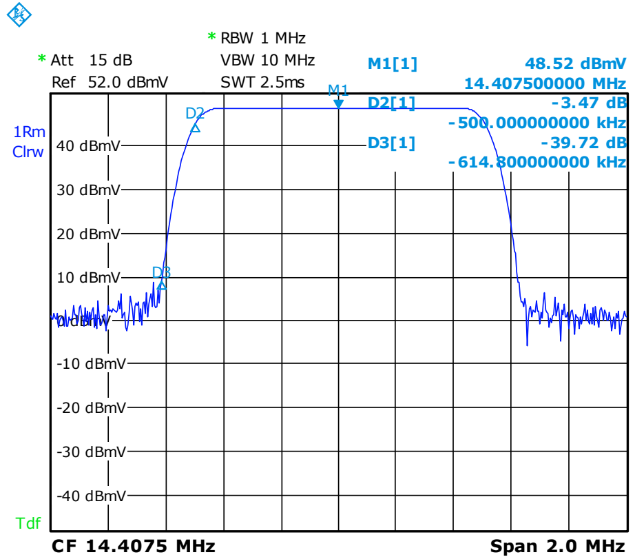
Fig. 15 Channel filter with 1 MHz bandwidth
