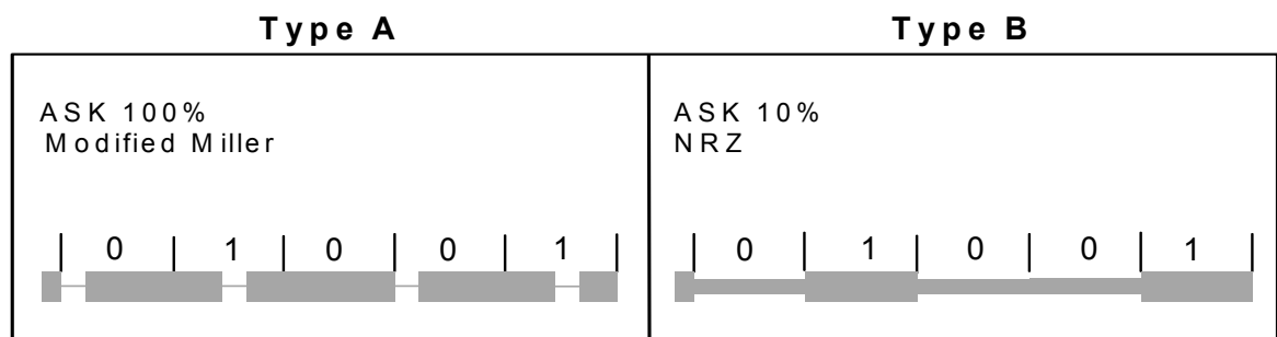
Fig. 1 PCD-to-PICC communication
