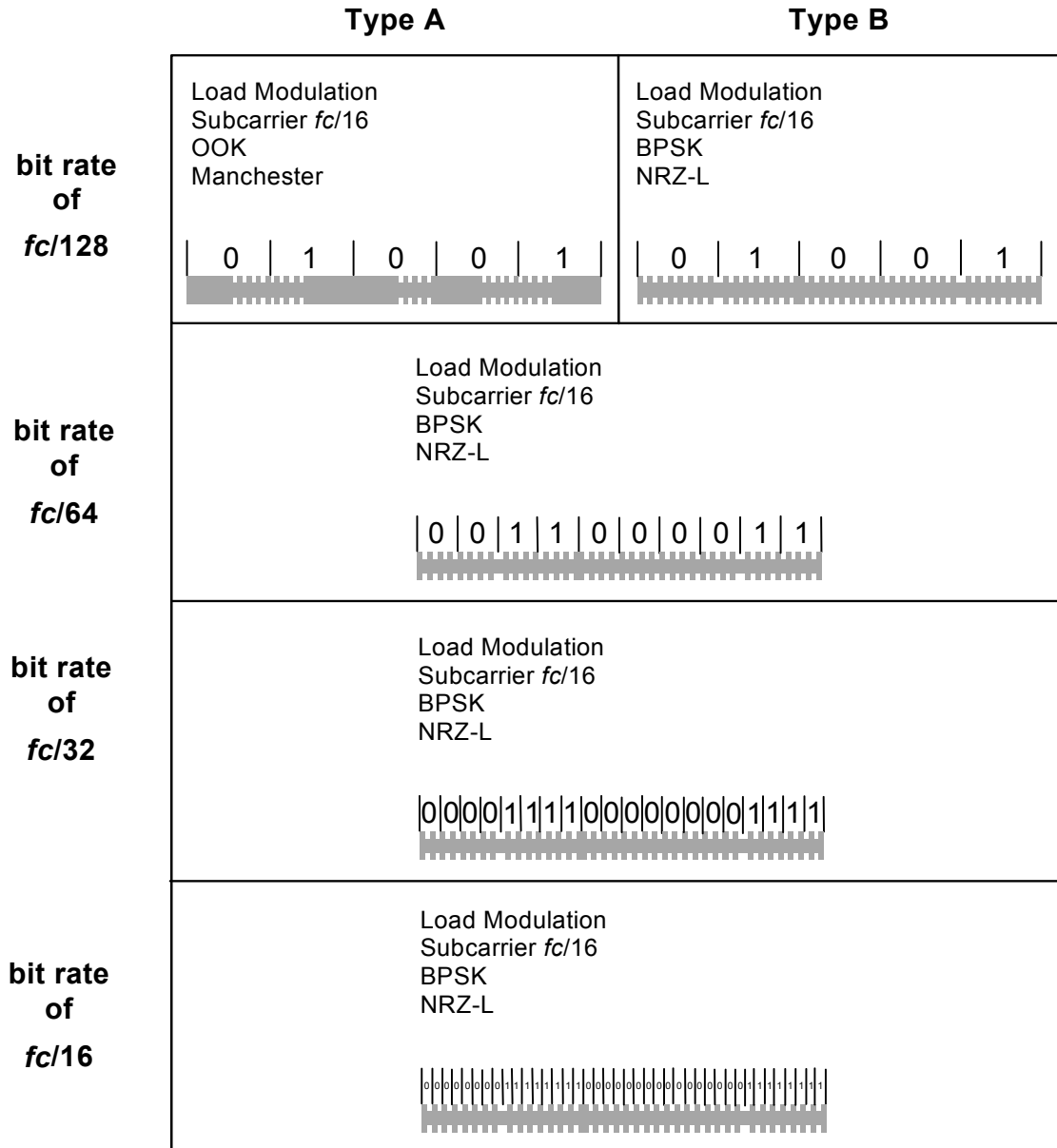
Fig. 2 PICC-to-PCD communication
