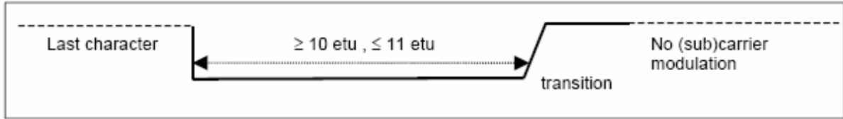
Fig. 28 Type B - end of frame
