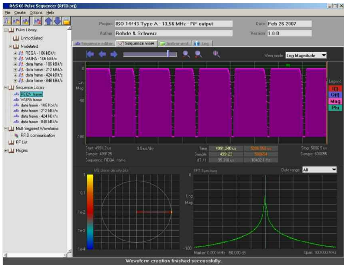
Fig. 19 R&S@xxx-K6 pulse sequencer - sequence view
