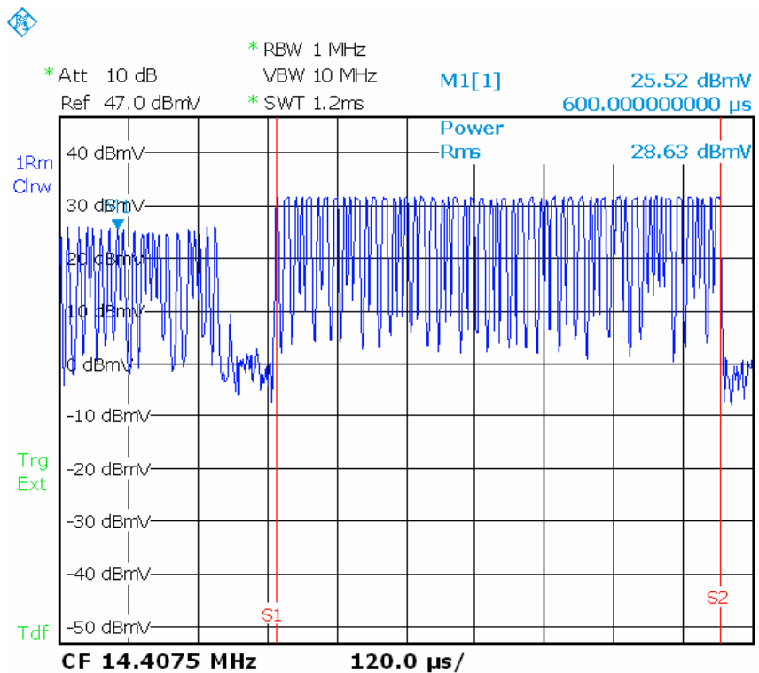
Fig. 16 Measurement - time domain power of load modulation (ISO/IEC 14443 Type A 106kbit/s)
