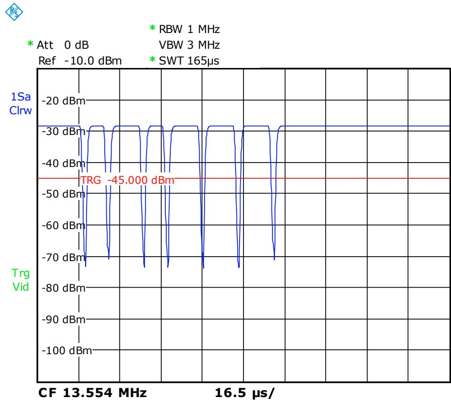
Fig. 26 Generated REQA frame measured with the R&S®FSL
