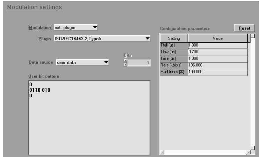
Fig. 20 Modulation settings of the ISO/IEC 14443 Type A plugin
