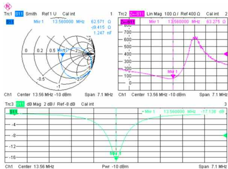
Fig. 6 s_{11} measurement of the PCD using an R&S@ZVL
