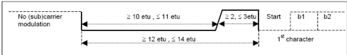
Fig. 27 Type B - start of frame
