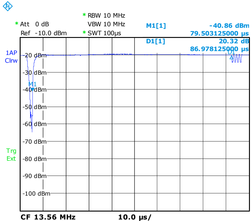
Fig. 13: Measuring the frame delay time (ISO/IEC 14443 Type A 106 kbit/s)
